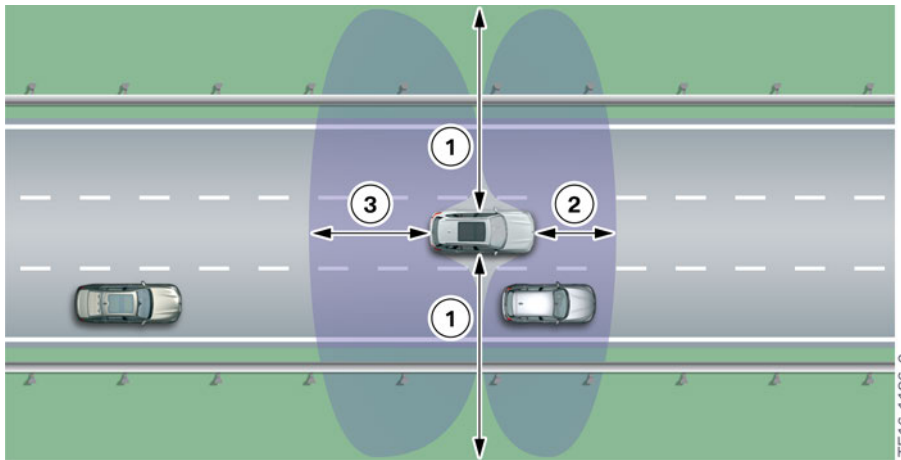
G05 sensor monitoring range for stationary objects (roadside structures) to the sides
