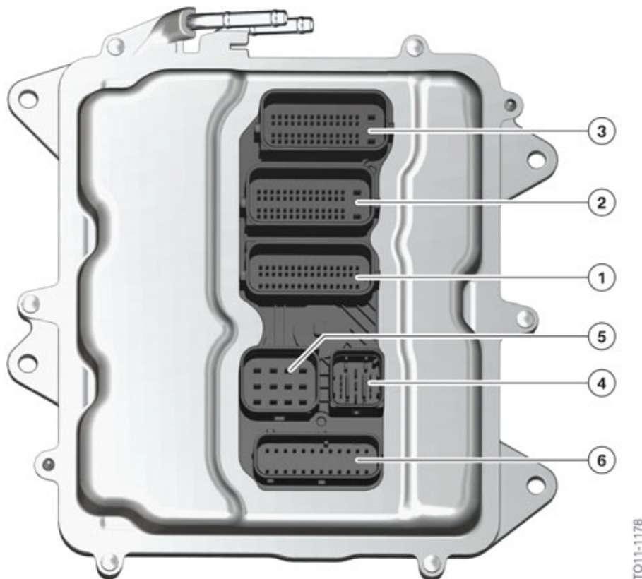
N63TU, MEVD17.2.8 DME connections
